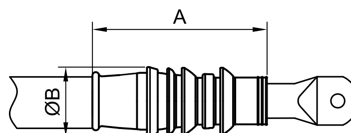
15 - CSTO-MK1 & 25 - CSTO-MK1
